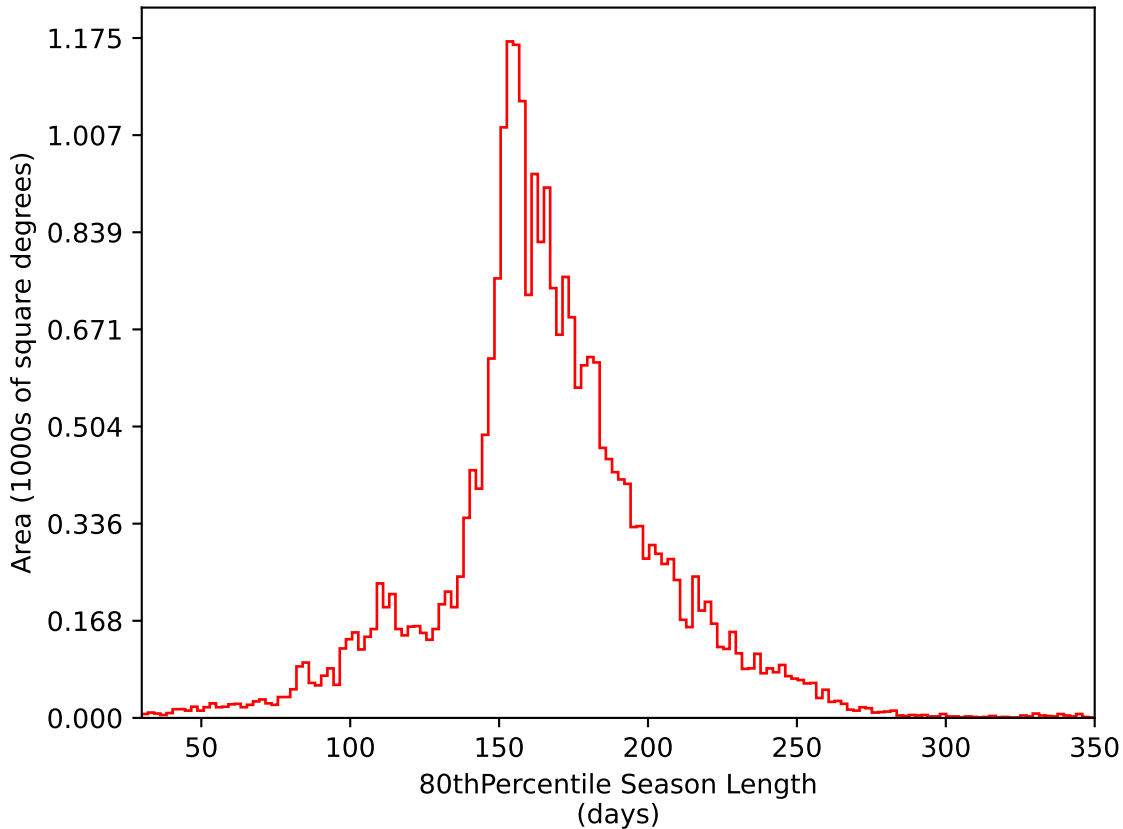
weather_cloudso8v3.4_10yrs All sky i band: 80thPercentile Season Length
