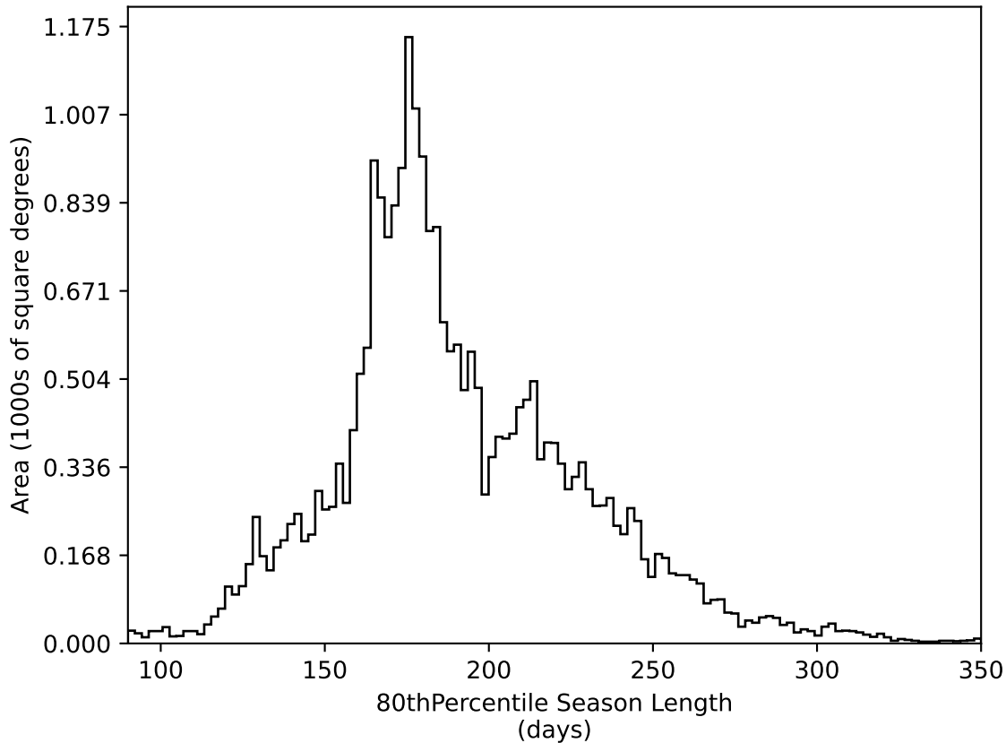
weather_cloudso8v3.4_10yrs All sky all bands: 80thPercentile Season Length
