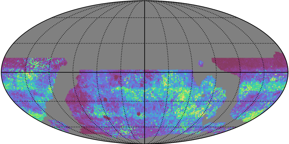
weather_cloudso8v3.4_10yrs WFD zy bands: 75th Percentile Intranight Timespan
