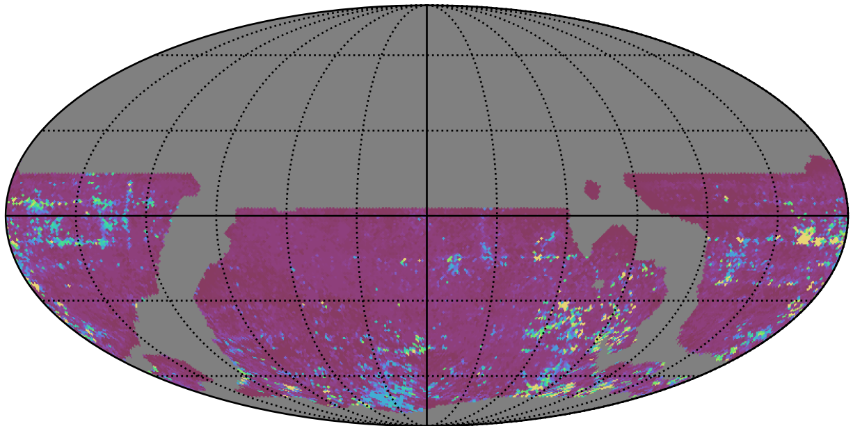
weather_cloudso8v3.4_10yrs WFD z band: 75th Percentile Intranight Timespan
