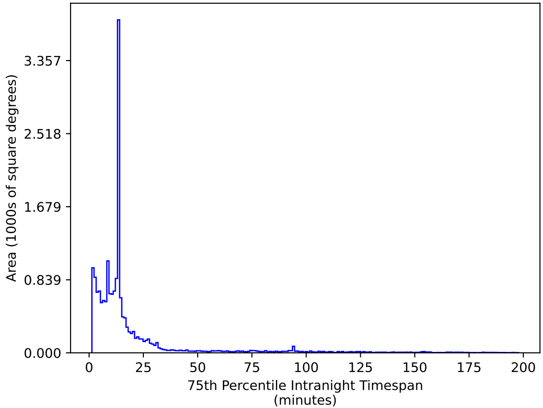
weather_cloudso8v3.4_10yrs WFD z band: 75th Percentile Intranight Timespan
