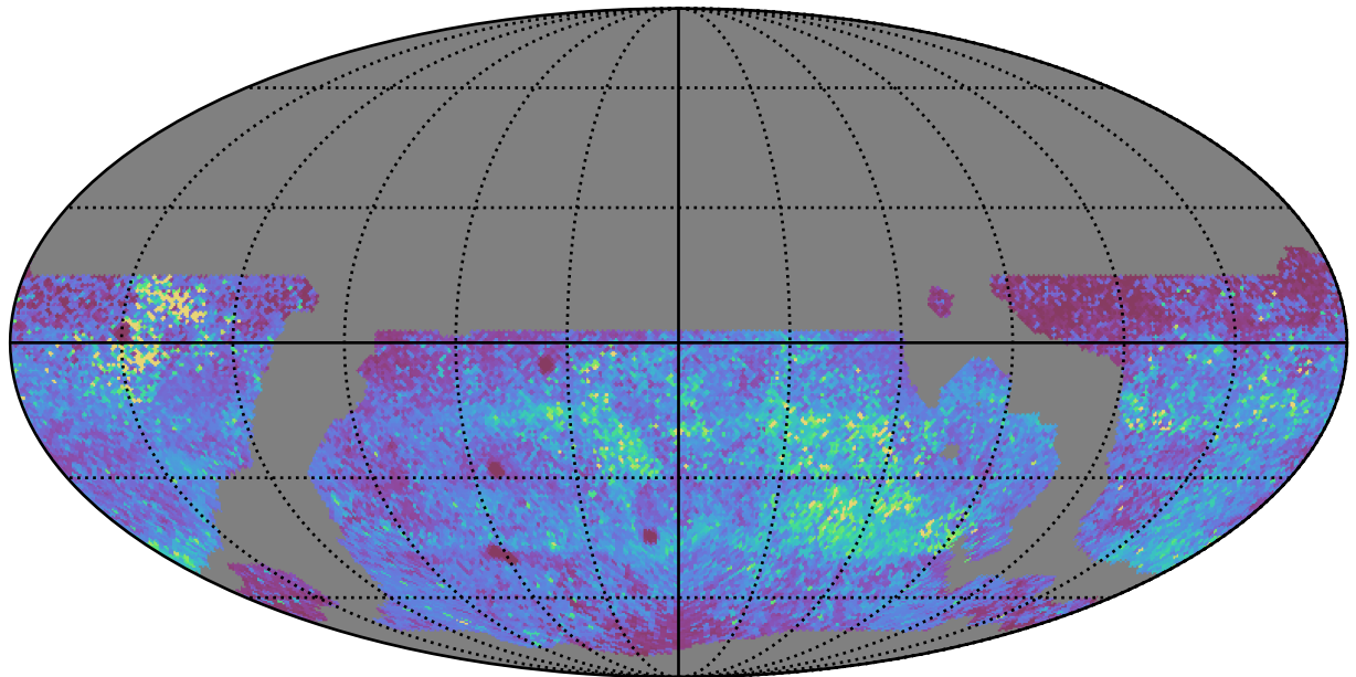
weather_cloudso8v3.4_10yrs WFD y band: 75th Percentile Intranight Timespan
