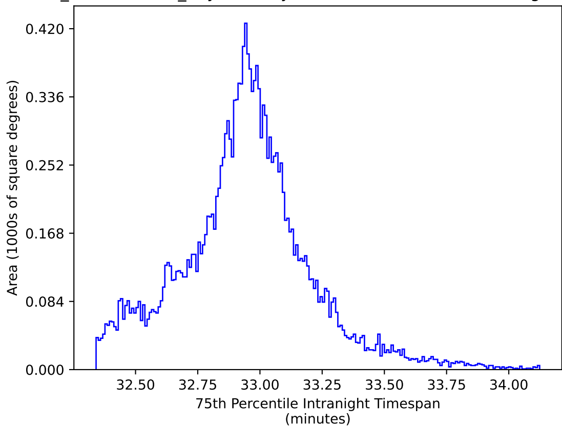
weather_cloudso8v3.4_10yrs WFD y band: 75th Percentile Intranight Timespan
