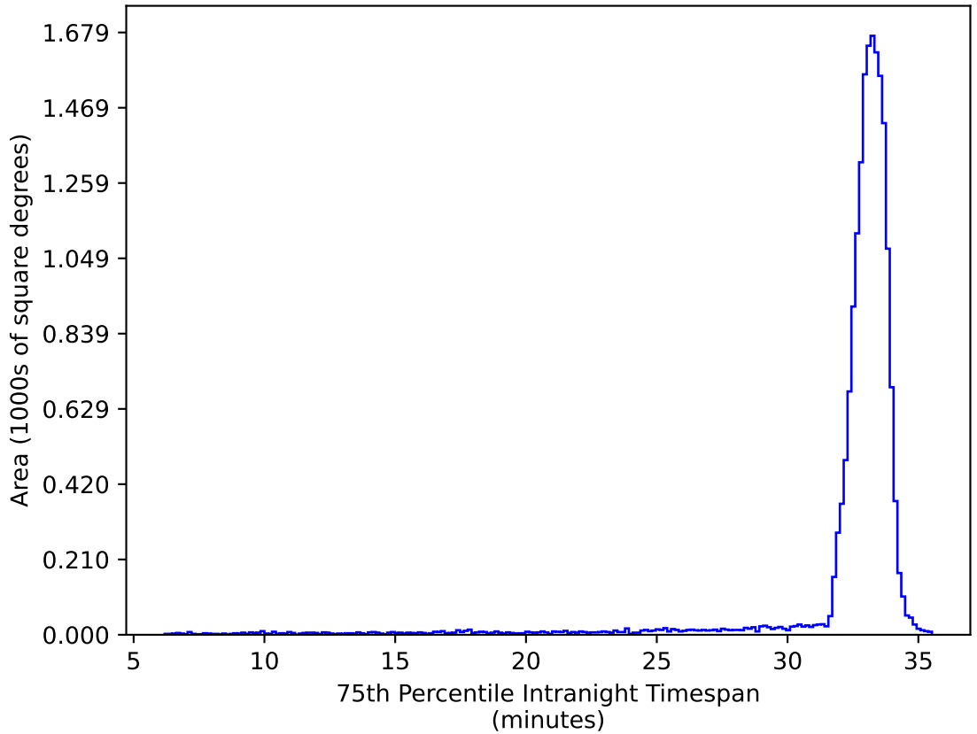
weather_cloudso8v3.4_10yrs WFD ug bands: 75th Percentile Intranight Timespan
