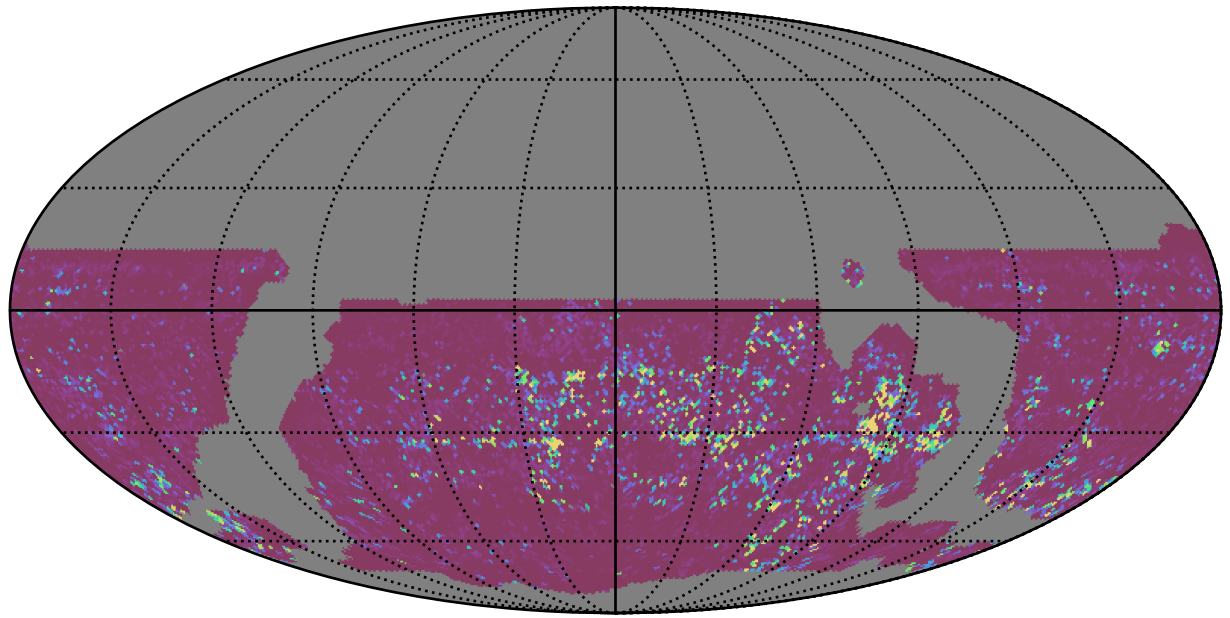
weather_cloudso8v3.4_10yrs WFD u band: 75th Percentile Intranight Timespan
