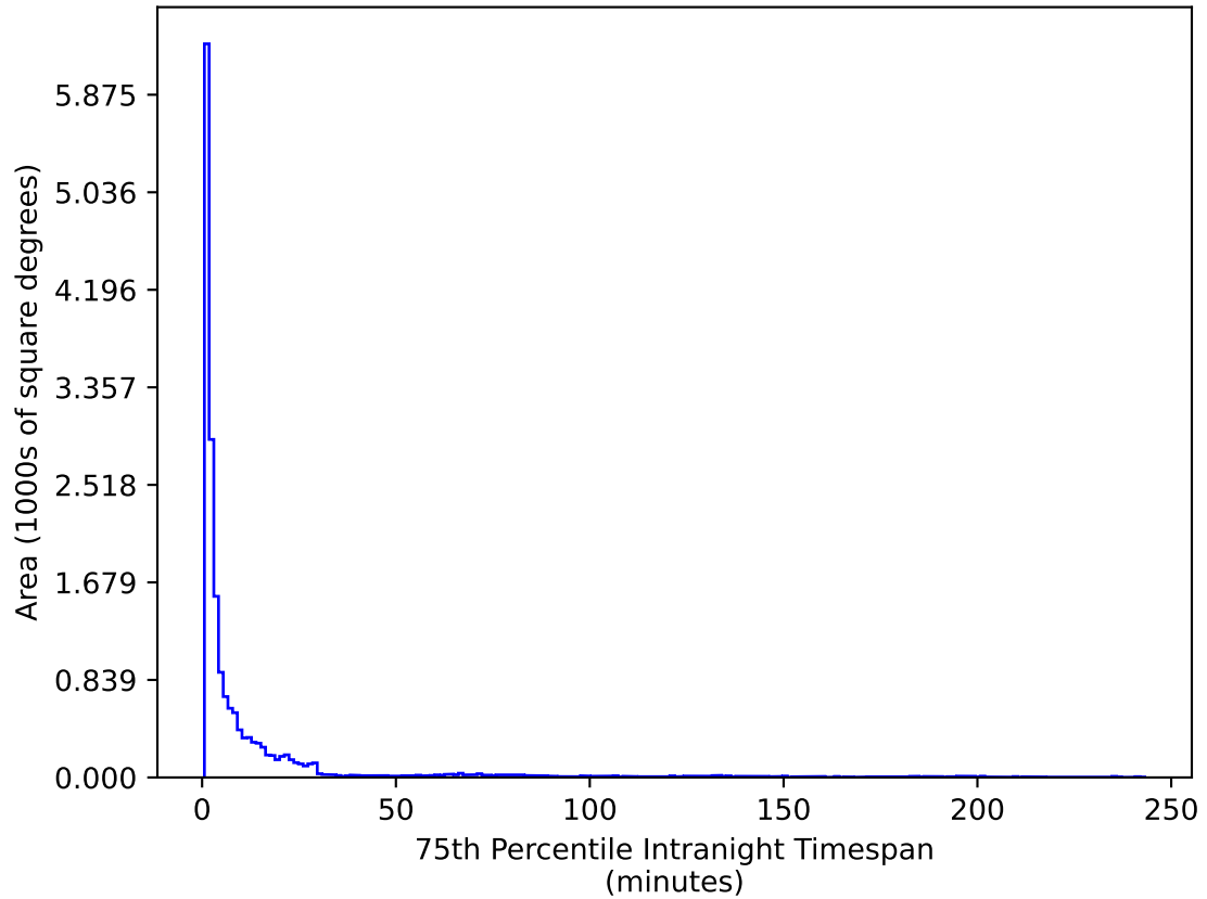
weather_cloudso8v3.4_10yrs WFD u band: 75th Percentile Intranight Timespan
