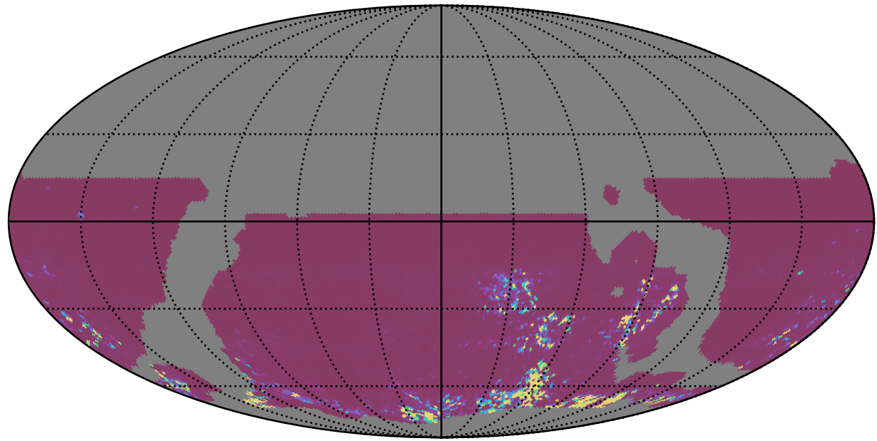
weather_cloudso8v3.4_10yrs WFD ri bands: 75th Percentile Intranight Timespan
