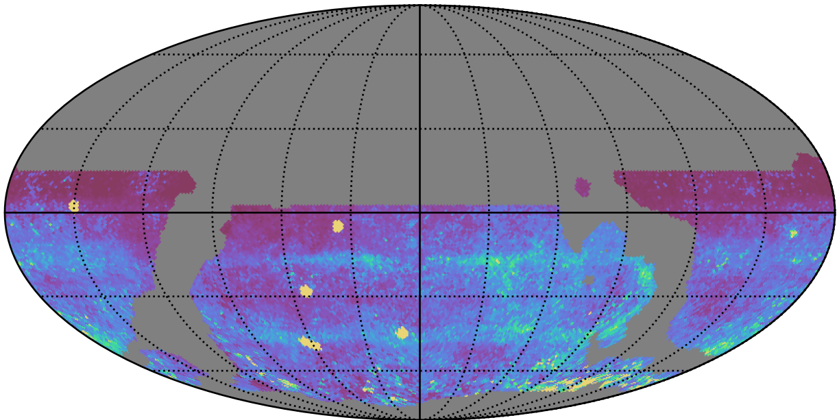
weather_cloudso8v3.4_10yrs WFD iz bands: 75th Percentile Intranight Timespan
