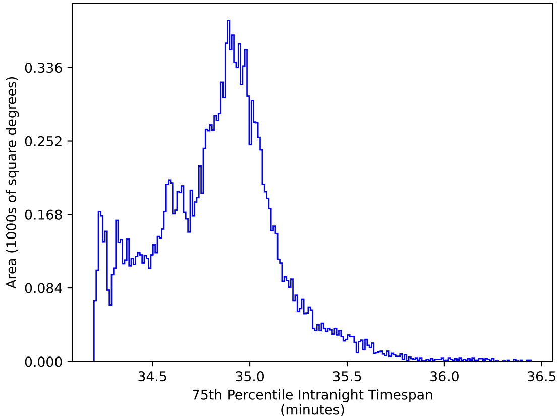
weather_cloudso8v3.4_10yrs WFD iz bands: 75th Percentile Intranight Timespan
