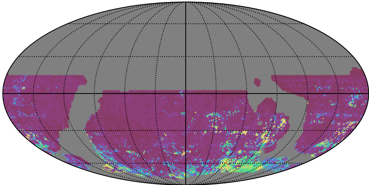
weather_cloudso8v3.4_10yrs WFD i band: 75th Percentile Intranight Timespan
