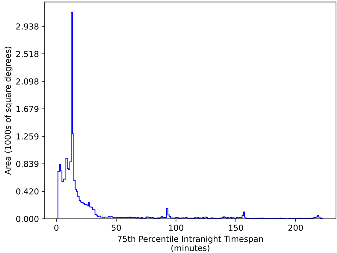
weather_cloudso8v3.4_10yrs WFD i band: 75th Percentile Intranight Timespan
