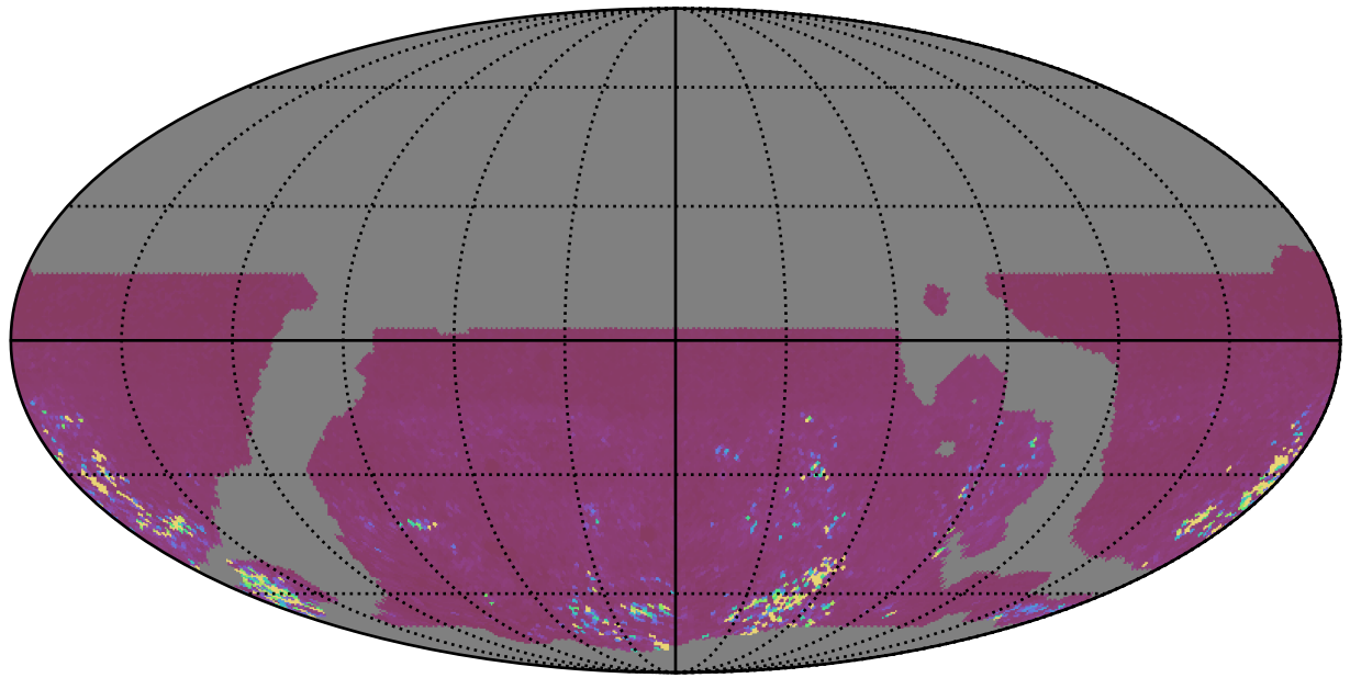
weather_cloudso8v3.4_10yrs WFD gr bands: 75th Percentile Intranight Timespan
