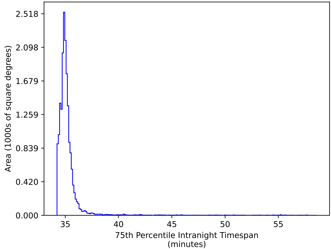
weather_cloudso8v3.4_10yrs WFD gr bands: 75th Percentile Intranight Timespan
