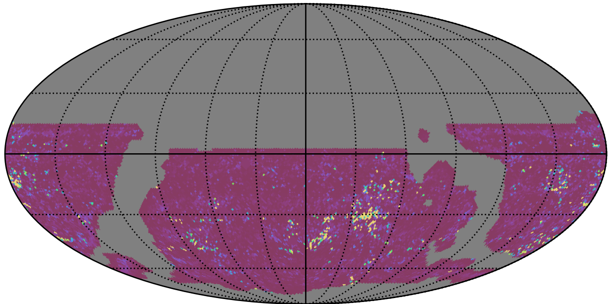
weather_cloudso8v3.4_10yrs WFD g band: 75th Percentile Intranight Timespan
