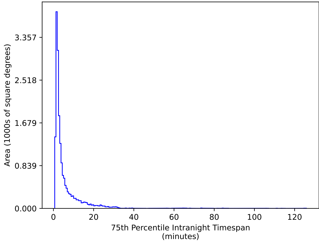
weather_cloudso8v3.4_10yrs WFD g band: 75th Percentile Intranight Timespan
