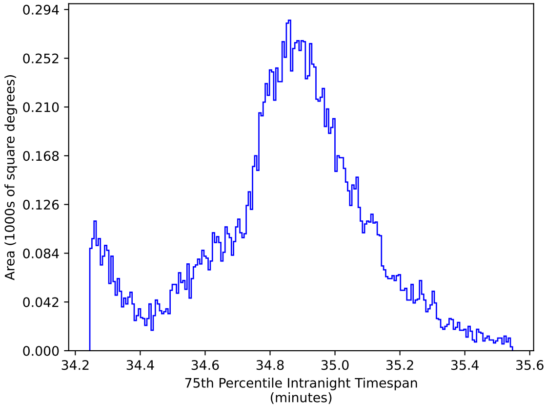
weather_cloudso8v3.4_10yrs WFD: 75th Percentile Intranight Timespan
