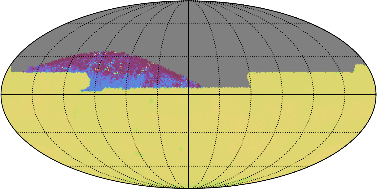
weather_cloudso8v3.4_10yrs All sky zy bands: 75th Percentile Intranight Timespan
