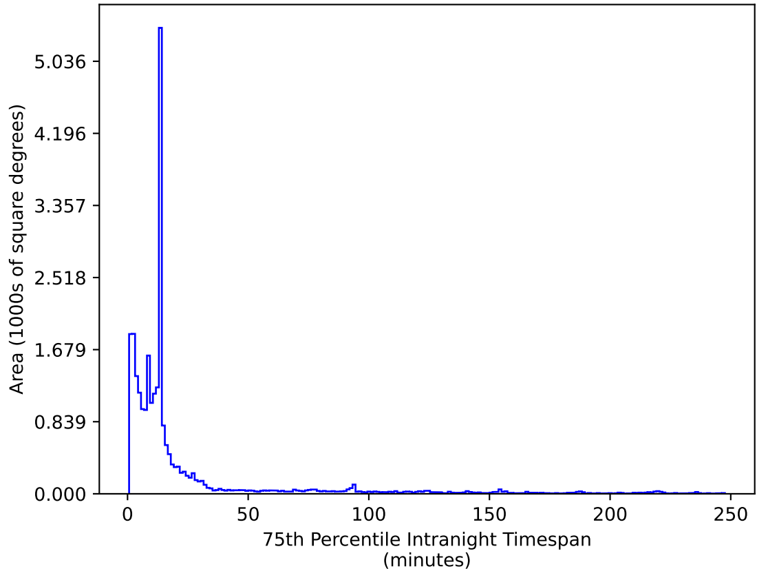
weather_cloudso8v3.4_10yrs All sky z band: 75th Percentile Intranight Timespan
