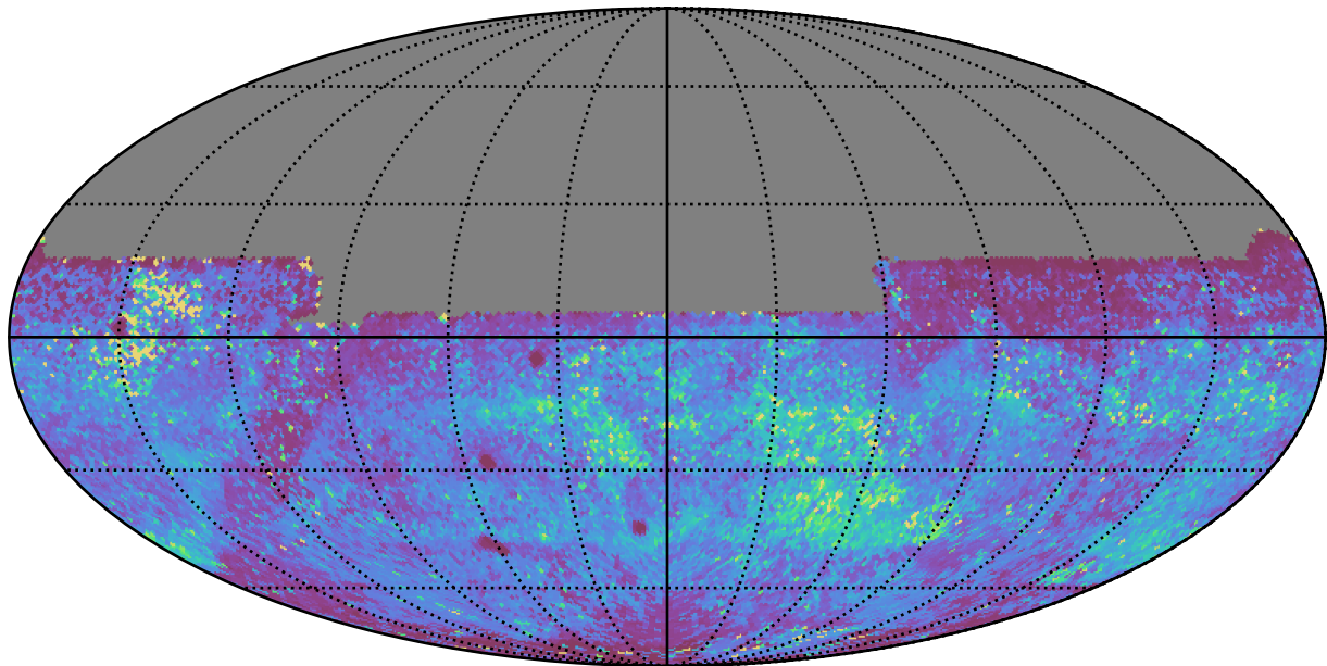
weather_cloudso8v3.4_10yrs All sky y band: 75th Percentile Intranight Timespan
