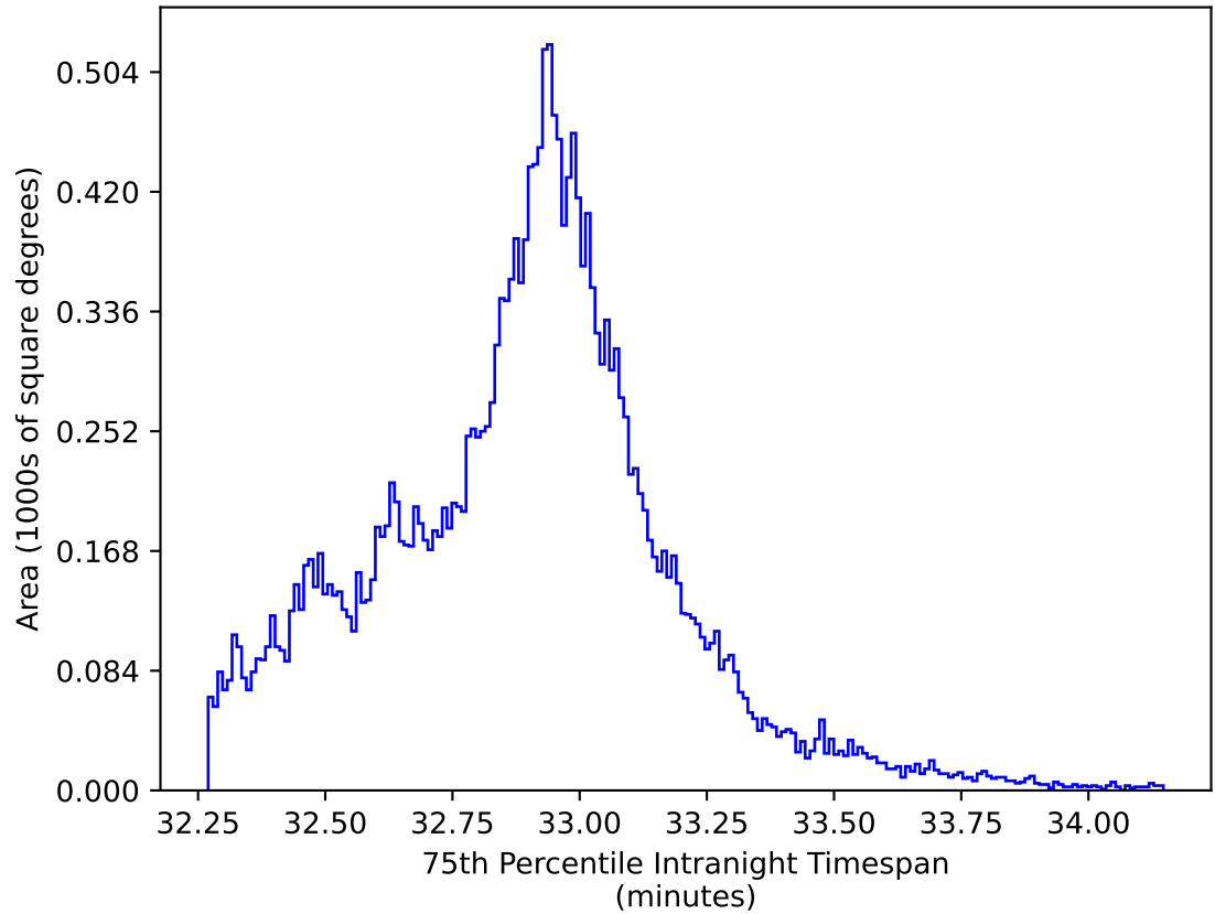
weather_cloudso8v3.4_10yrs All sky y band: 75th Percentile Intranight Timespan
