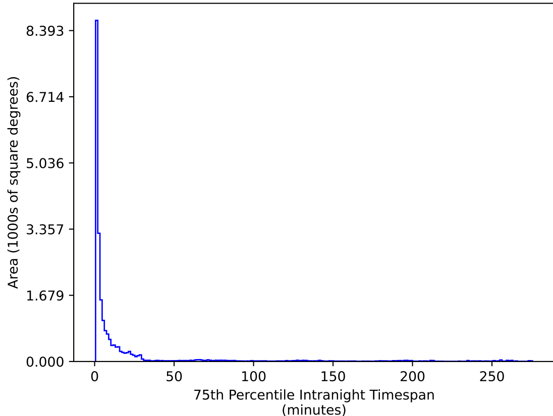
weather_cloudso8v3.4_10yrs All sky u band: 75th Percentile Intranight Timespan
