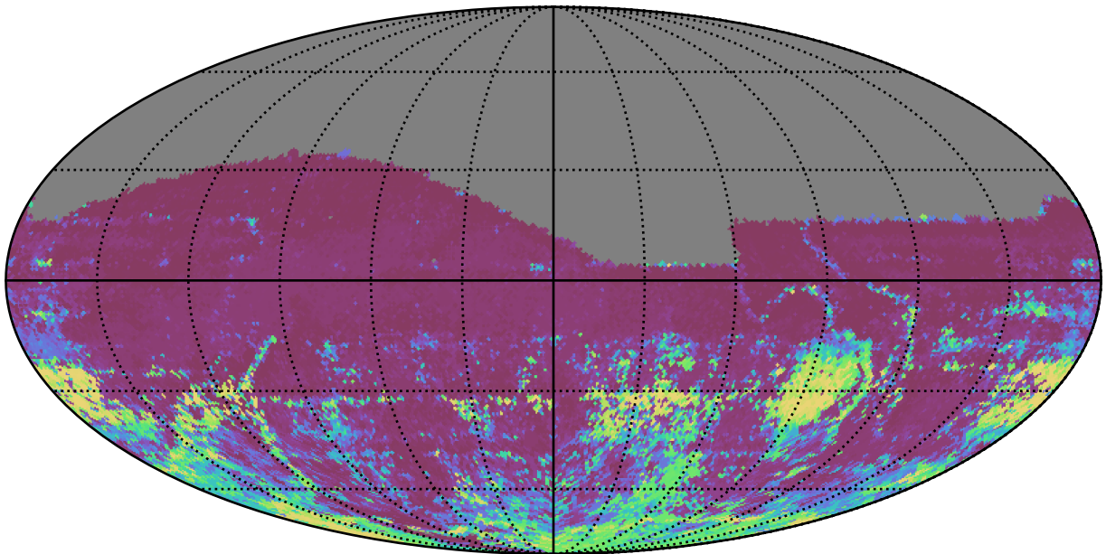
weather_cloudso8v3.4_10yrs All sky r band: 75th Percentile Intranight Timespan
