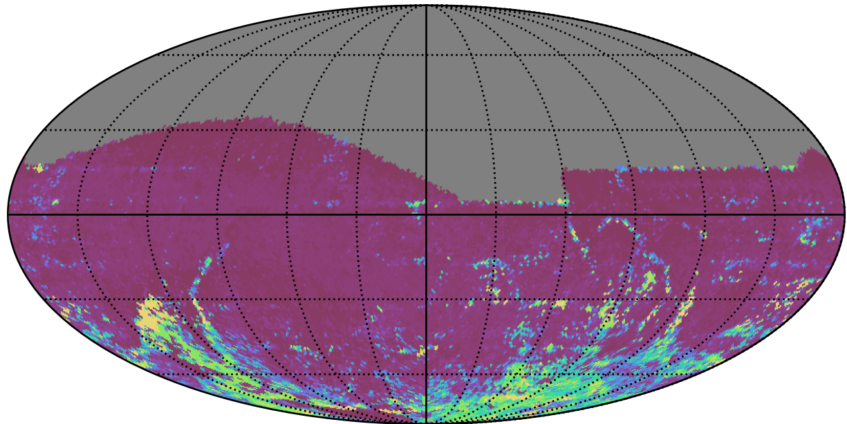
weather_cloudso8v3.4_10yrs All sky i band: 75th Percentile Intranight Timespan
