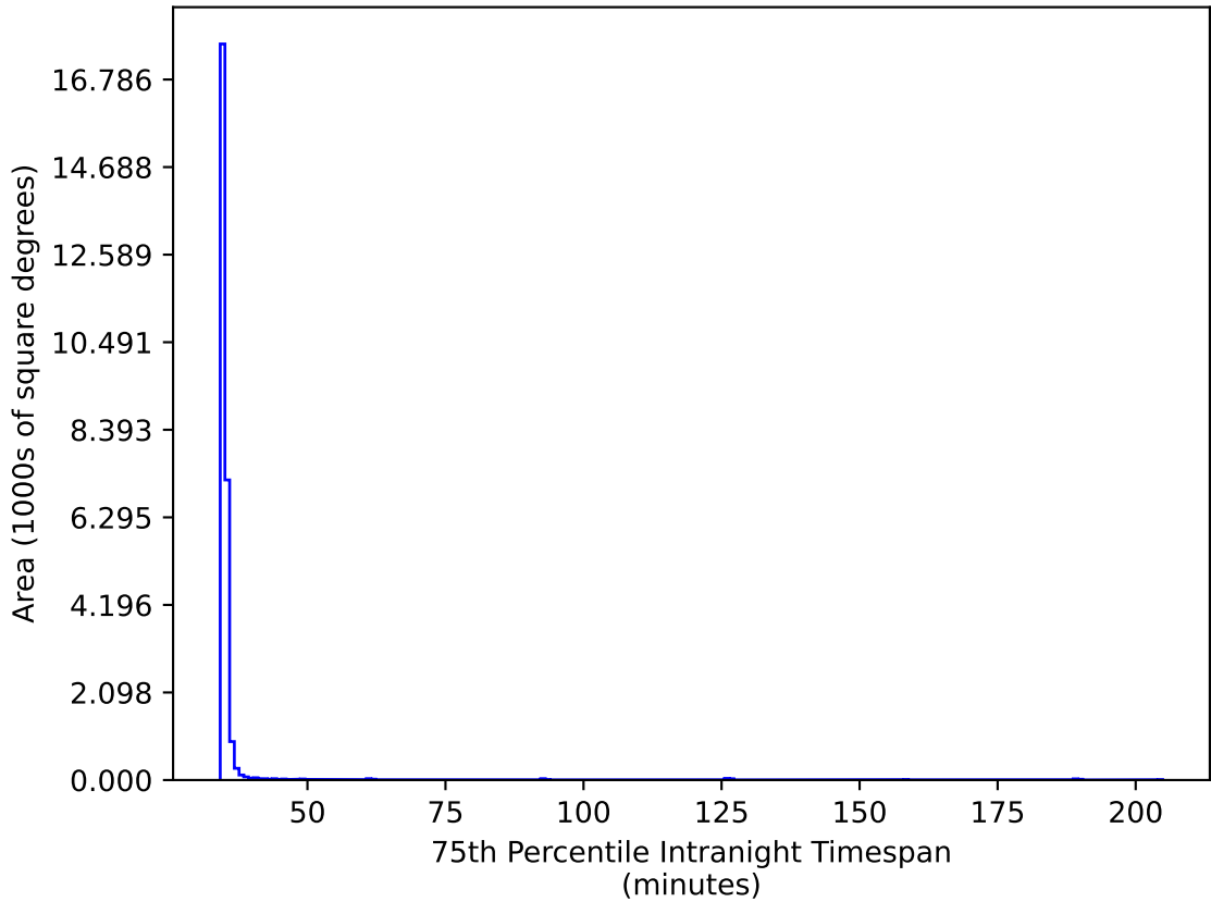
weather_cloudso8v3.4_10yrs All sky gr bands: 75th Percentile Intranight Timespan
