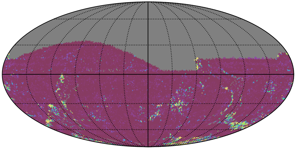
weather_cloudso8v3.4_10yrs All sky g band: 75th Percentile Intranight Timespan
