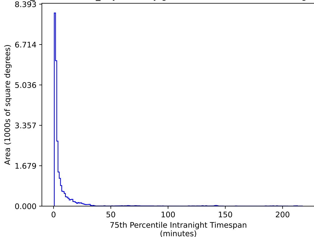
weather_cloudso8v3.4_10yrs All sky g band: 75th Percentile Intranight Timespan
