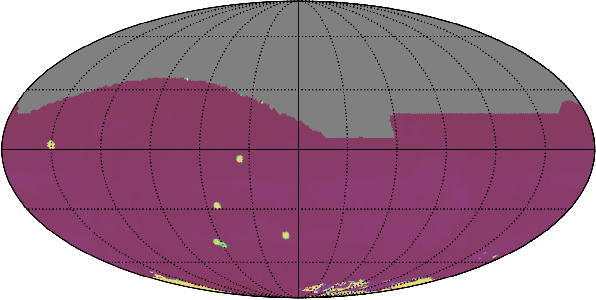
weather_cloudso8v3.4_10yrs All sky all bands: 75th Percentile Intranight Timespan
