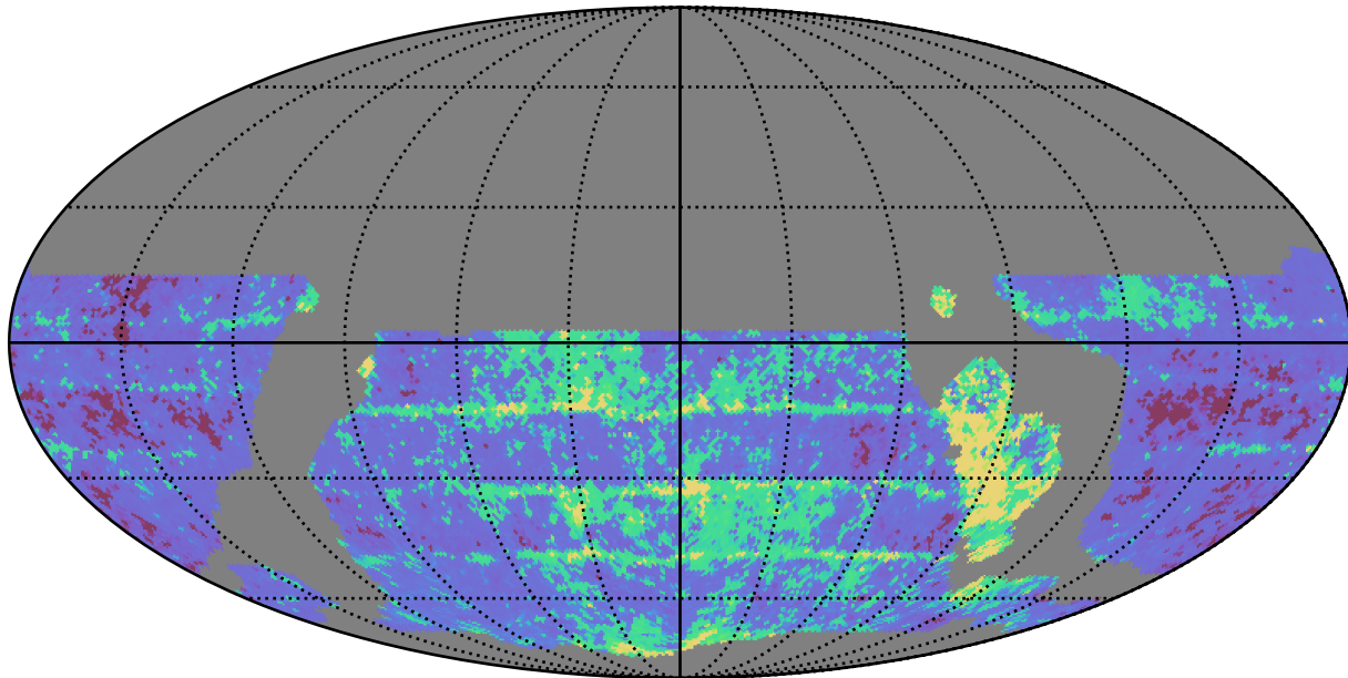
weather_cloudso8v3.4_10yrs WFD z band: 20thPercentile Inter-Night Gap
