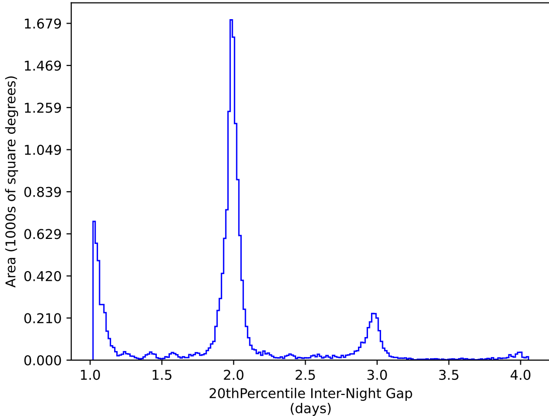
weather_cloudso8v3.4_10yrs WFD y band: 20thPercentile Inter-Night Gap
