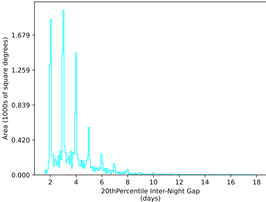
weather_cloudso8v3.4_10yrs WFD u band: 20thPercentile Inter-Night Gap
