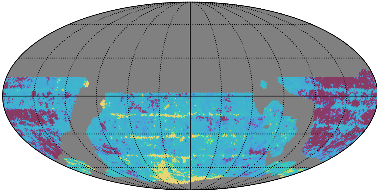
weather_cloudso8v3.4_10yrs WFD r band: 20thPercentile Inter-Night Gap
