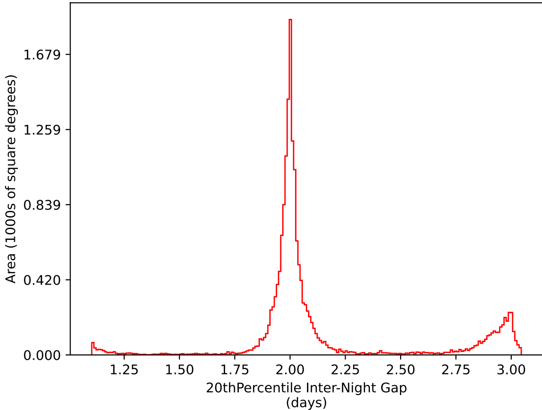
weather_cloudso8v3.4_10yrs WFD i band: 20thPercentile Inter-Night Gap
