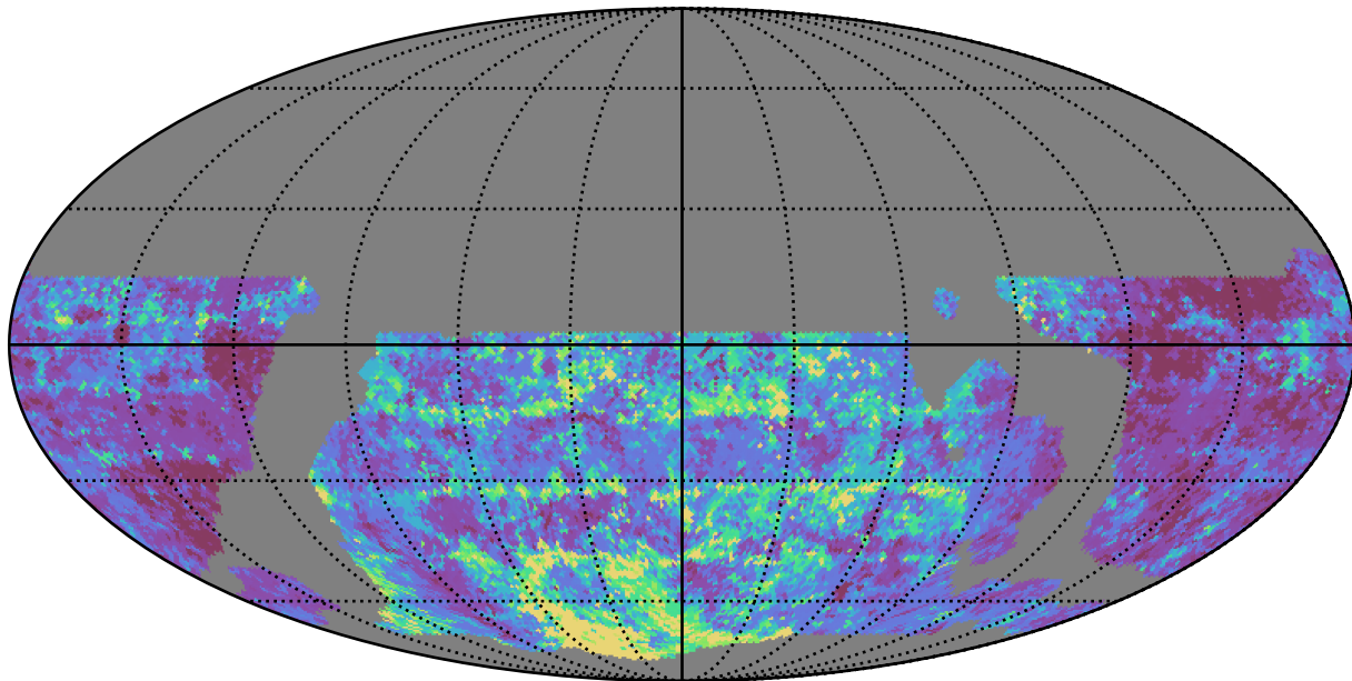
weather_cloudso8v3.4_10yrs WFD g band: 20thPercentile Inter-Night Gap
