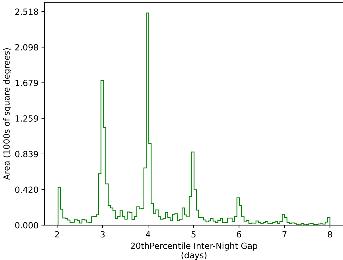
weather_cloudso8v3.4_10yrs WFD g band: 20thPercentile Inter-Night Gap
