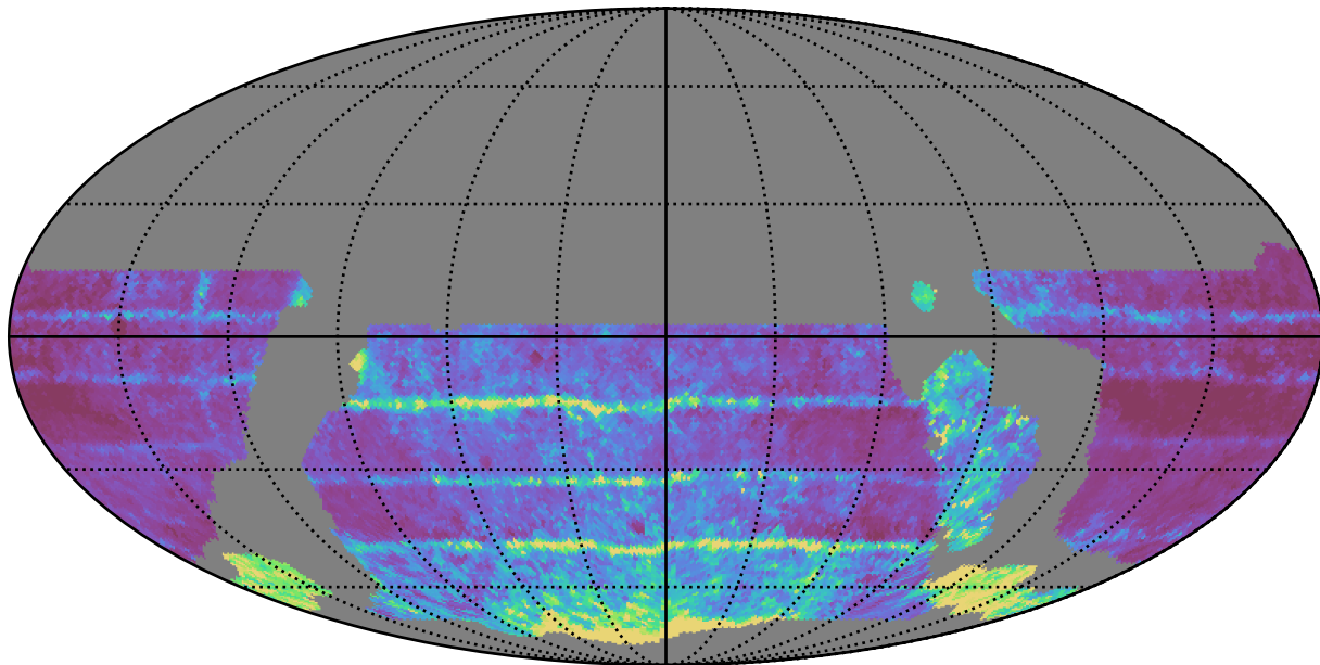
weather_cloudso8v3.4_10yrs WFD all bands: 20thPercentile Inter-Night Gap
