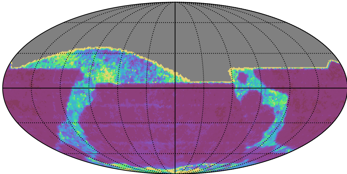
weather_cloudso8v3.4_10yrs All sky i band: 20thPercentile Inter-Night Gap
