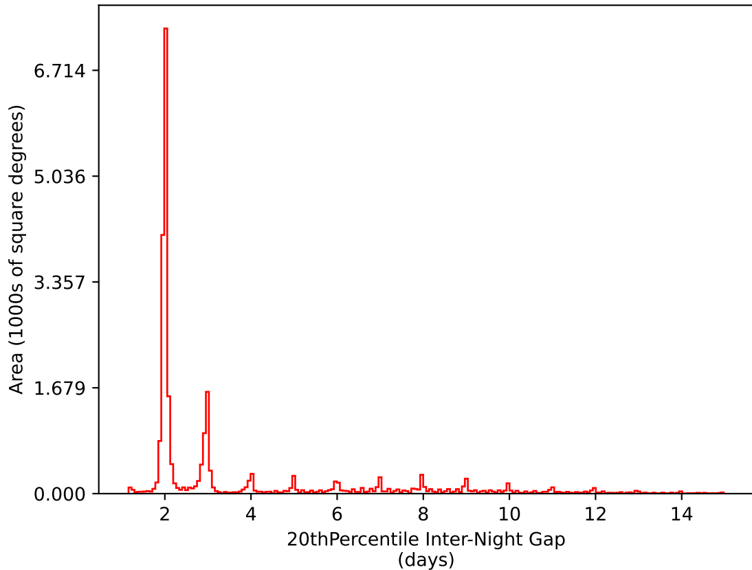
weather_cloudso8v3.4_10yrs All sky i band: 20thPercentile Inter-Night Gap
