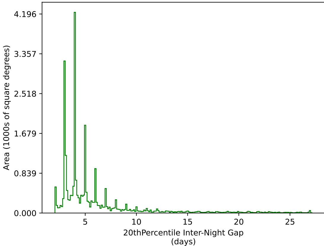
weather_cloudso8v3.4_10yrs All sky g band: 20thPercentile Inter-Night Gap
