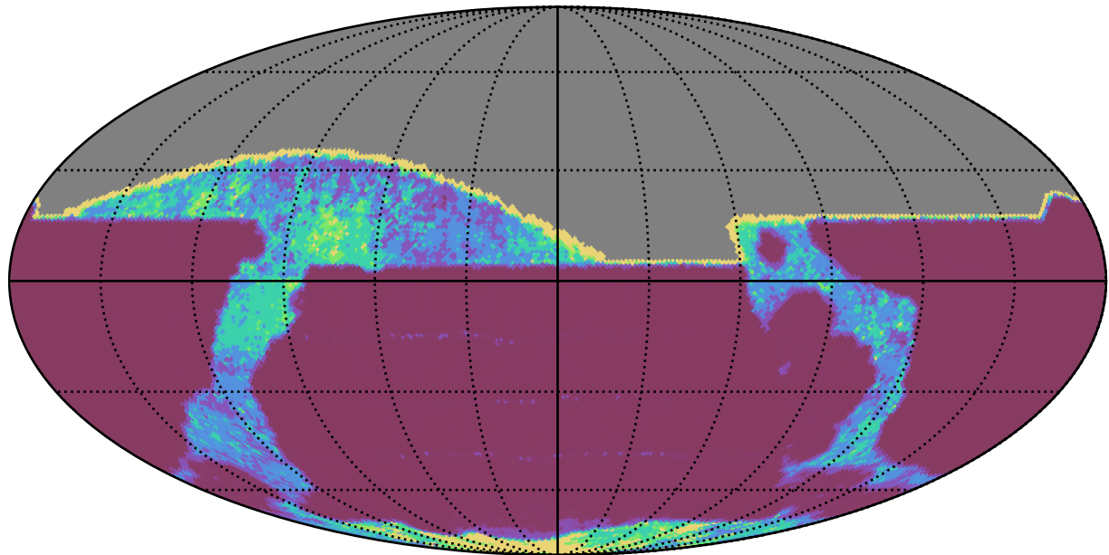
weather_cloudso8v3.4_10yrs All sky all bands: 20thPercentile Inter-Night Gap
