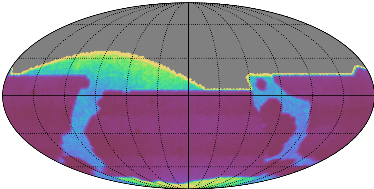
weather_cloudso8v3.4_10yrs : properMotion
