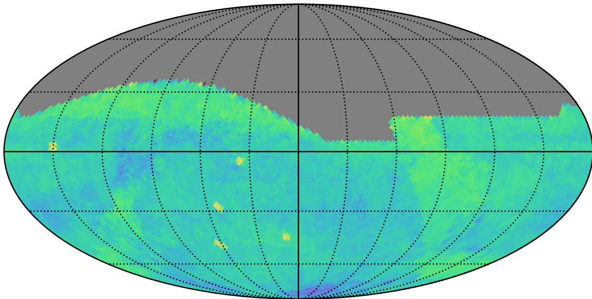
weather_cloudso8v3.4_10yrs (g or r or i): PairFraction
