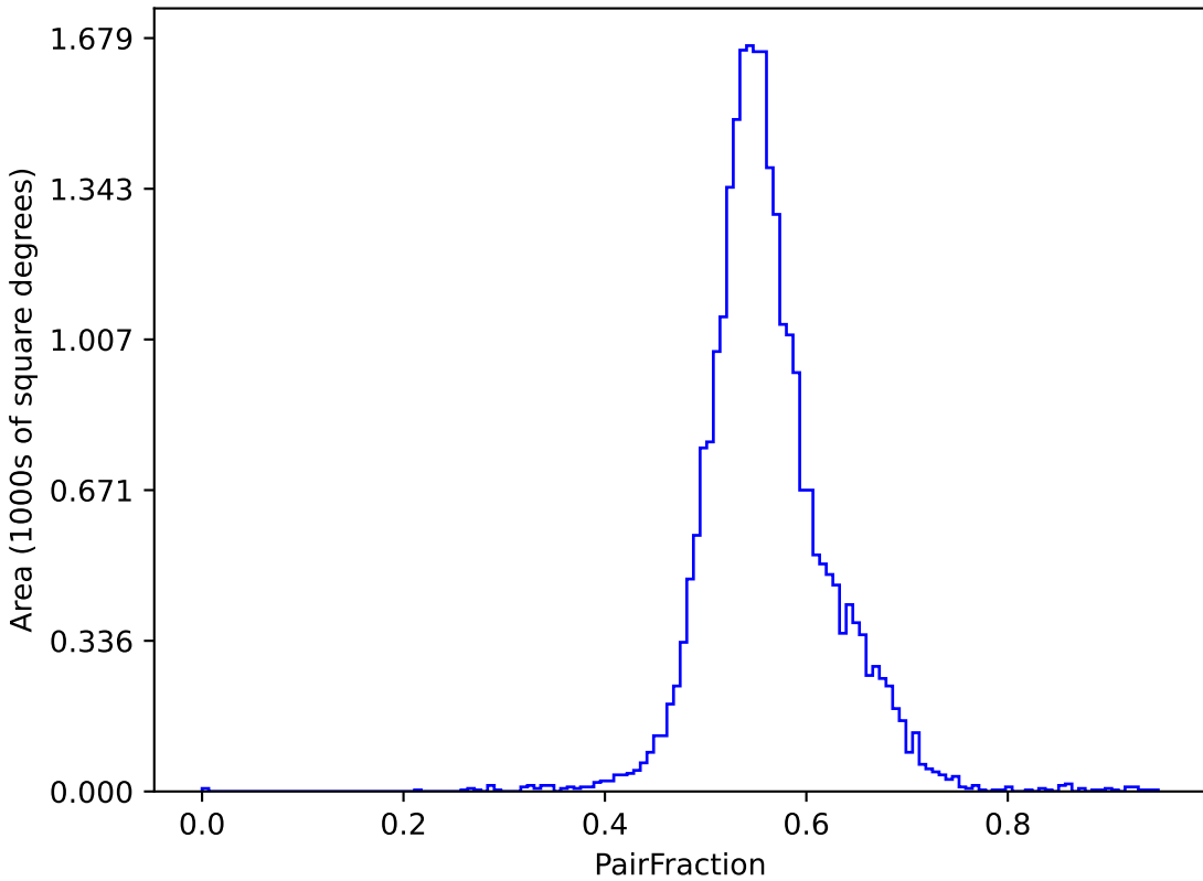
weather_cloudso8v3.4_10yrs (g or r or i): PairFraction
