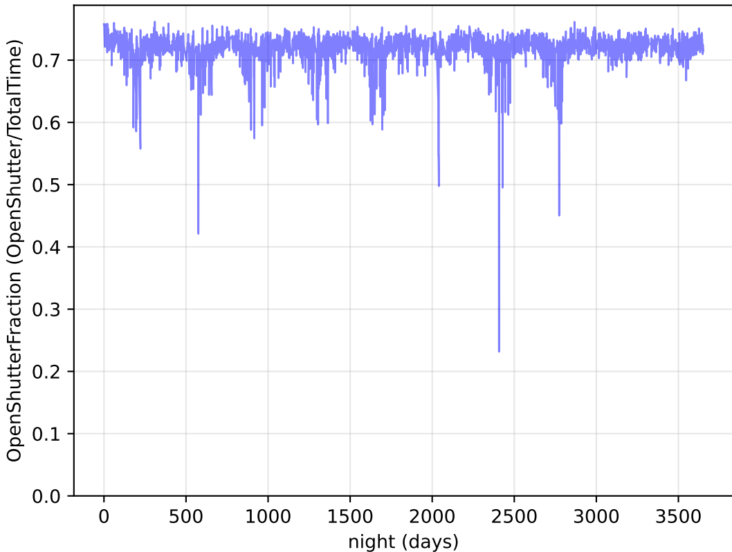
weather_cloudso8v3.4_10yrs : OpenShutterFraction
