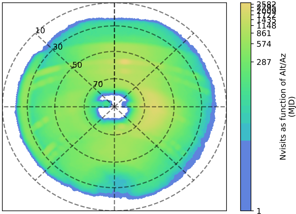
weather_cloudso8v3.4_10yrs r: Nvisits as function of Alt/Az
