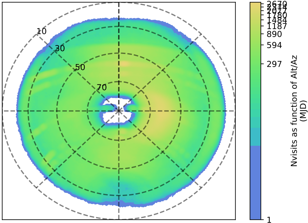
weather_cloudso8v3.4_10yrs i: Nvisits as function of Alt/Az
