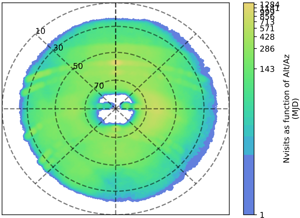
weather_cloudso8v3.4_10yrs g: Nvisits as function of Alt/Az
